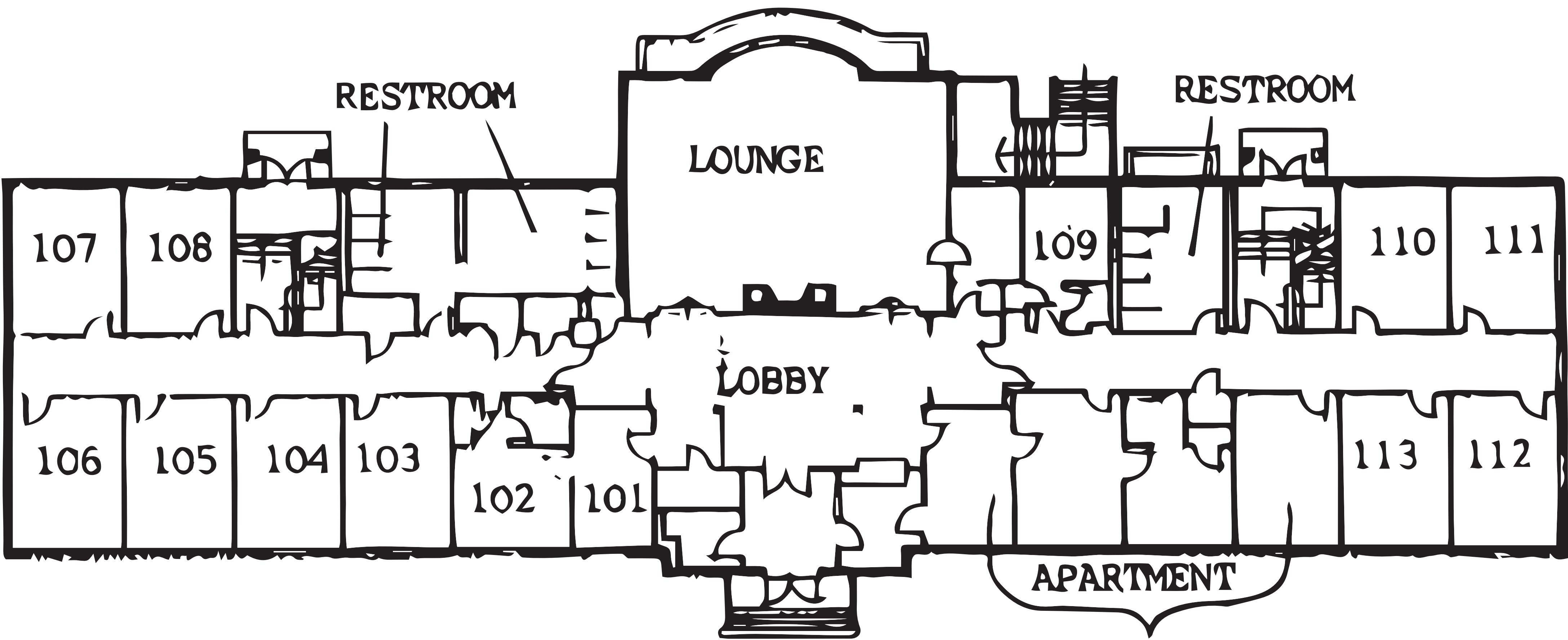
FIRST FLOOR
